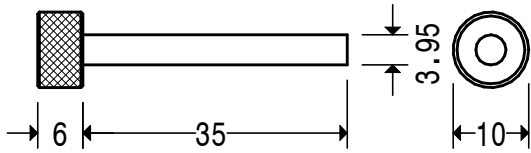
MATERIAL 10 DIA. STEEL 230M07 QTY 2 OFF SPINDLE 2
