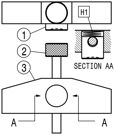
H1 SMALL COMPRESSION SPRING. MINI DEPTH GAUGE
