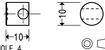
HOLE 4 MATERIAL 10 DIA. STEEL 230M07 QTY 2 OFF SEE TEXT RE POSITIONING THE HOLE AND LENGTH MAKE HEAD SLIGHTLY CONCAVE. CLAMP 1
