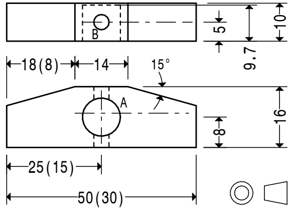
HOLES A 10 B 4 MATERIAL 16 X 10 STEEL 070M20 QTY 1 OFF MAKE A SECOND BASE USING DIMENSIONS IN ( ) BASE 3
