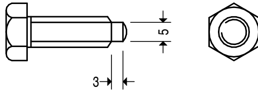
CLAMP SCREW
