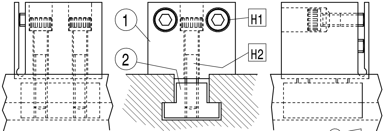
CLAMP JAW ASSEMBLY
