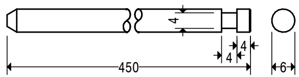
MATERIAL 6 DIAMETER STEEL 230M07 QTY. 1 OFF STOP BAR 8
