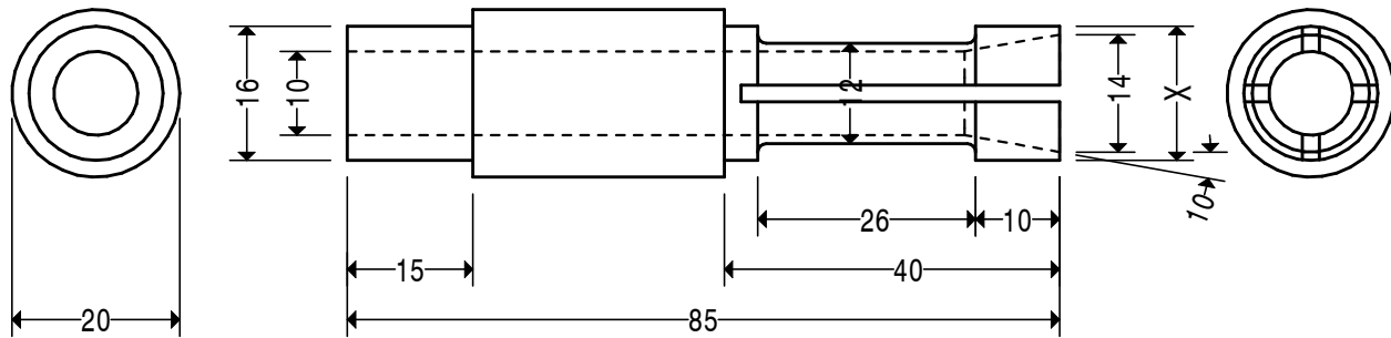
MATERIAL 20 DIAMETER STEEL 230M07 QTY. 1 OFF SEE TEXT RE DIMENSION X. SLIT COLLET END 40MM LONG 2MM WIDE X 4 AS SHOWN
