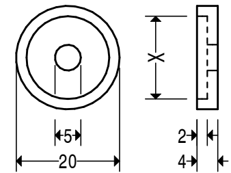
CUP WASHER FOR SECURING BODY WHILST SLITTING. SEE TEXT RE DIMENSION X CUP WASHER SK. 1
