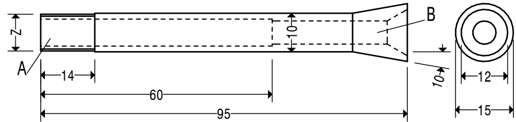
MATERIAL 16 DIAMETER STEEL 230M07 QTY. 1 OFF HOLES A. 7 B. 6 USE CENTRE DRILL TO PRODUCE TAPER ENTRY NOTE Z. 3/8" X 32 TPI ME THREAD
