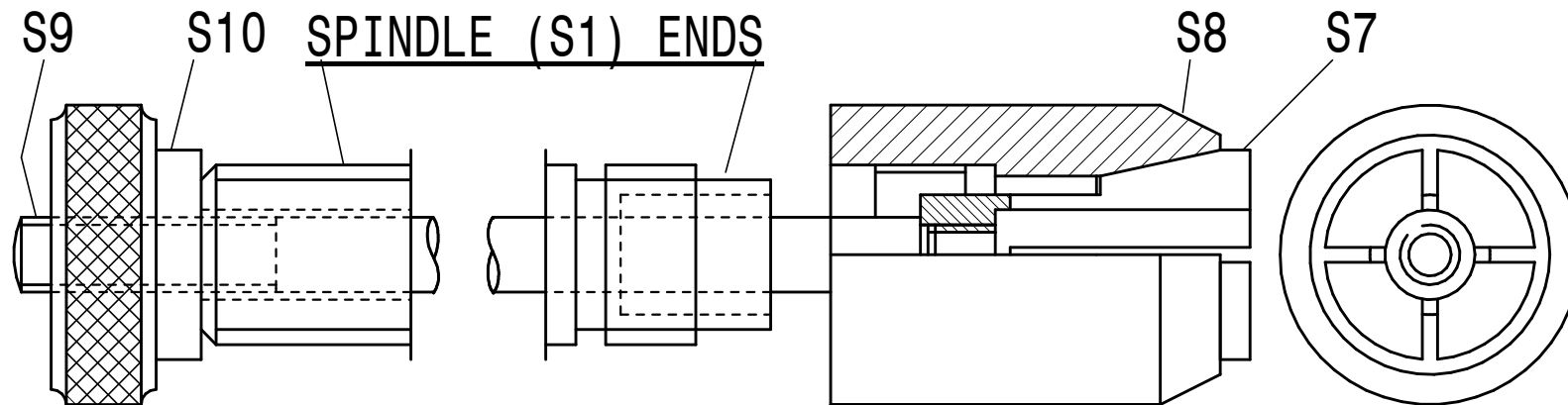
SMALL COLLET CHUCK ASSEMBLY AS6
