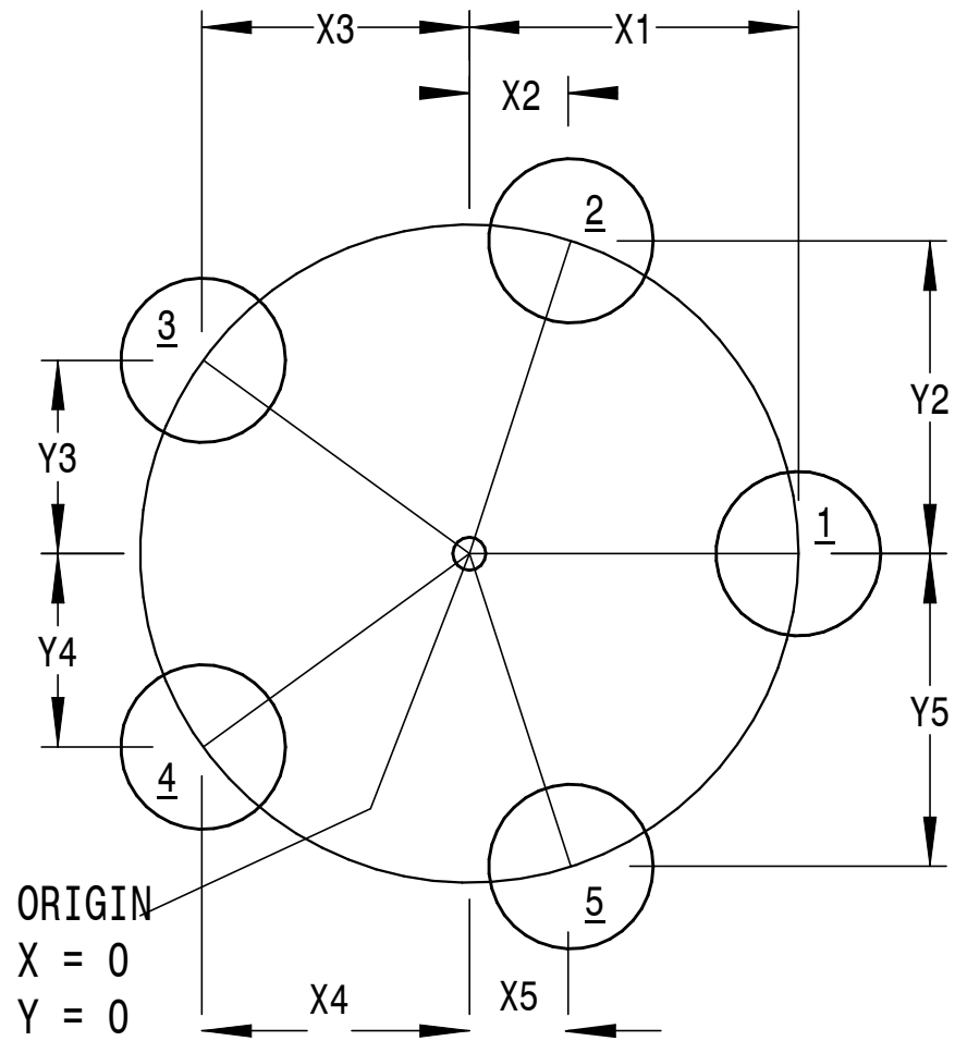
FIVE CIRCLES ON A PITCH CIRCLE DIAMETER ORIGIN AT CENTRE OF PITCH CIRCLE DIAMETER.
