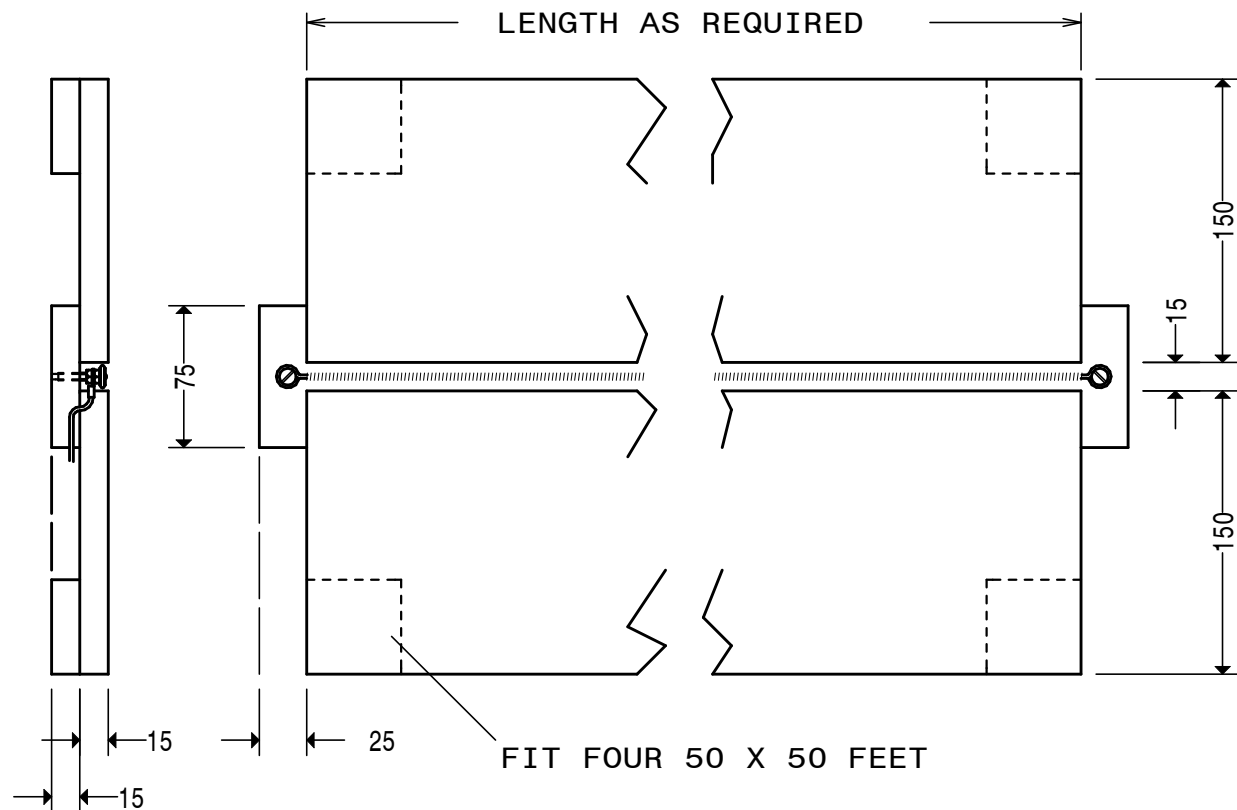
HOT WIRE PLASTIC SHEET BENDER SK1.
