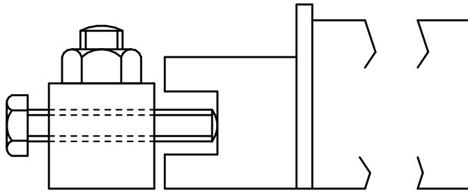
ALTERNATIVE CLAMP FOR PHOTO 20 SK.5
