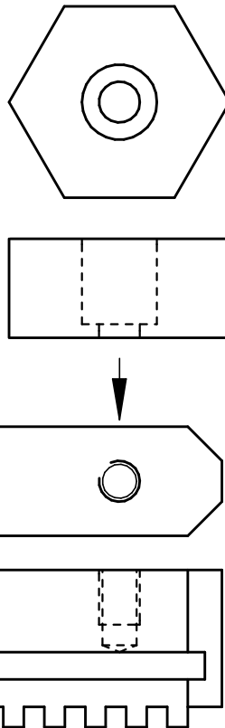
SIMPLIFIED HEXAGON JAWS
