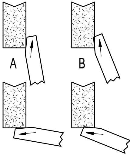
CORRECT TOOL APPROACH ANGLE SK.1 INCORRECT
