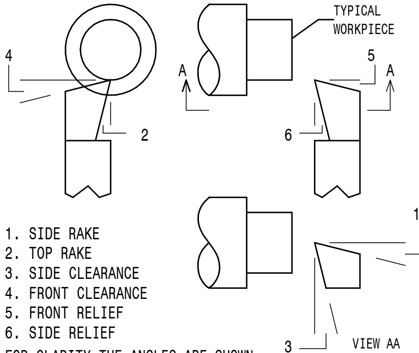
1. SIDE RAKE 2. TOP RAKE 3. SIDE CLEARANCE 4. FRONT CLEARANCE 5. FRONT RELIEF 6. SIDE RELIEF FOR CLARITY THE ANGLES ARE SHOWN GREATER THAN IS NORMALLY REQUIRED LATHE TOOL ANGLES SK.3
