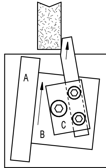
A. FENCE B. SWIVEL BASE C. SQUARE TOOL HOLDER SETUP FOR GRINDING A LATHE TOOL SK.2
