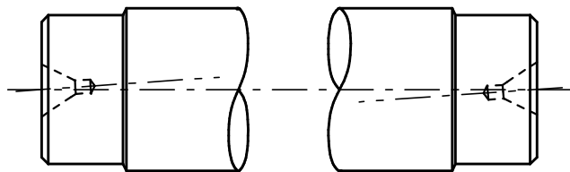
MISALIGNED CENTRES CAN OCCUR IF DRILLED ON THE DRILLING MACHINE. MISALIGNED CENTRES SK.2
