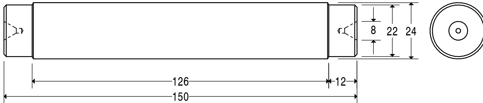
MATERIAL. 25mm DIAMETER 230M07 STEEL BETWEEN CENTRES PARALLEL TEST BAR. SK. 1
