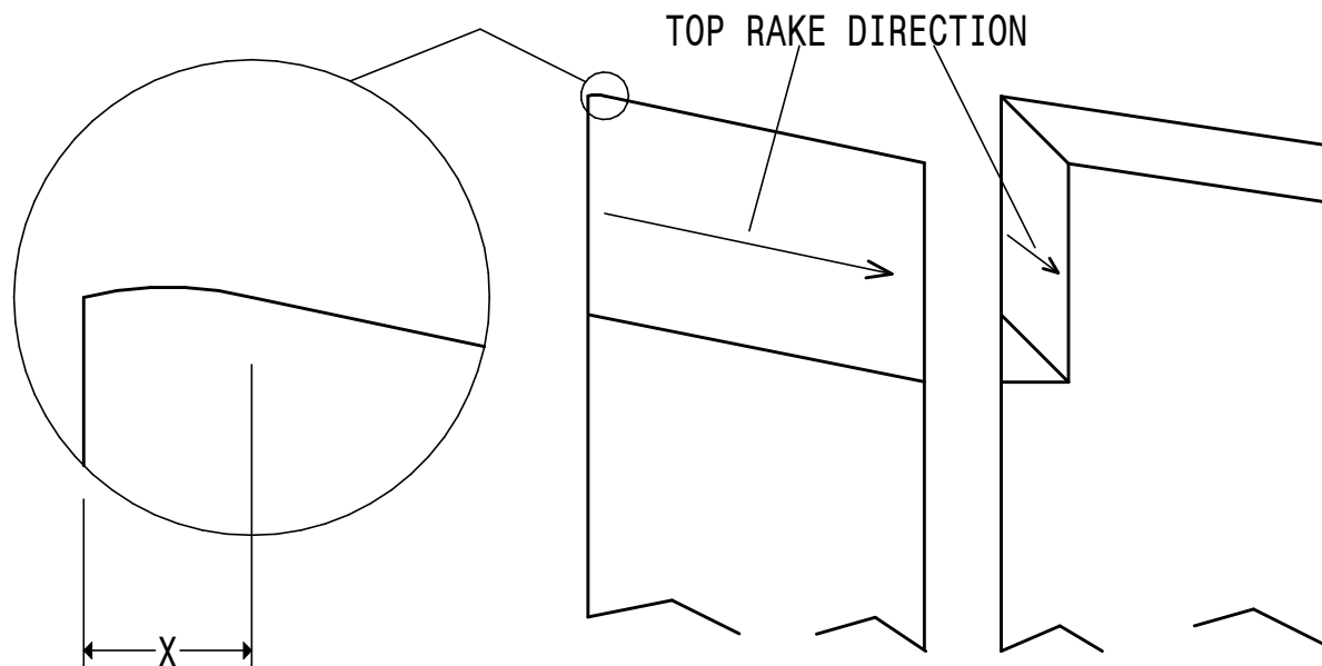
X. MAKE SLIGHT CURVE 0.2 TO 0.5MM WIDE CUTTER MUST BE HONED TO HAVE A FINE EDGE! KNIFE TOOL FOR FINISHING SK.3
